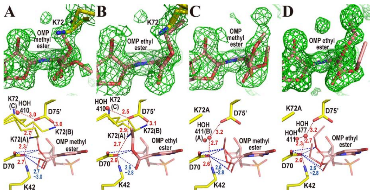
Figure 4. Methyl and ethyl ester complexes of ODCase. The upper panels show omit electron density maps superposed on the refined models. The omit electron density maps ( 2.0\sigma ) were phased without the atoms of the ligand and K72 included in the calculations. The lower panels display the binding modes of the ligands in detail. Red and blue numbers give distances in angstroms. (A) WT-MtODCase with OMP-methyl-ester. (B) WT-MtODCase with OMP-ethyl-ester. (C) K72A-MtODCase with OMP-methyl-ester. (D) K72A-MtODCase with OMP-ethyl-ester.
