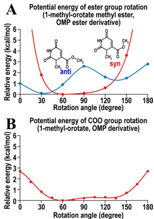
Figure 5. Potential energy profiles of the rotation around the C6–C7 bond of OMP analogues. (A) Profile of 1-methyl-orotate methyl ester, a model compound for OMP methyl ester. Blue and red lines indicate the profiles for anti and syn conformations of the methyl group, respectively, whose chemical formulas are also shown. (B) Profile of the carboxylate group rotation in 1-methyl-orotate.
