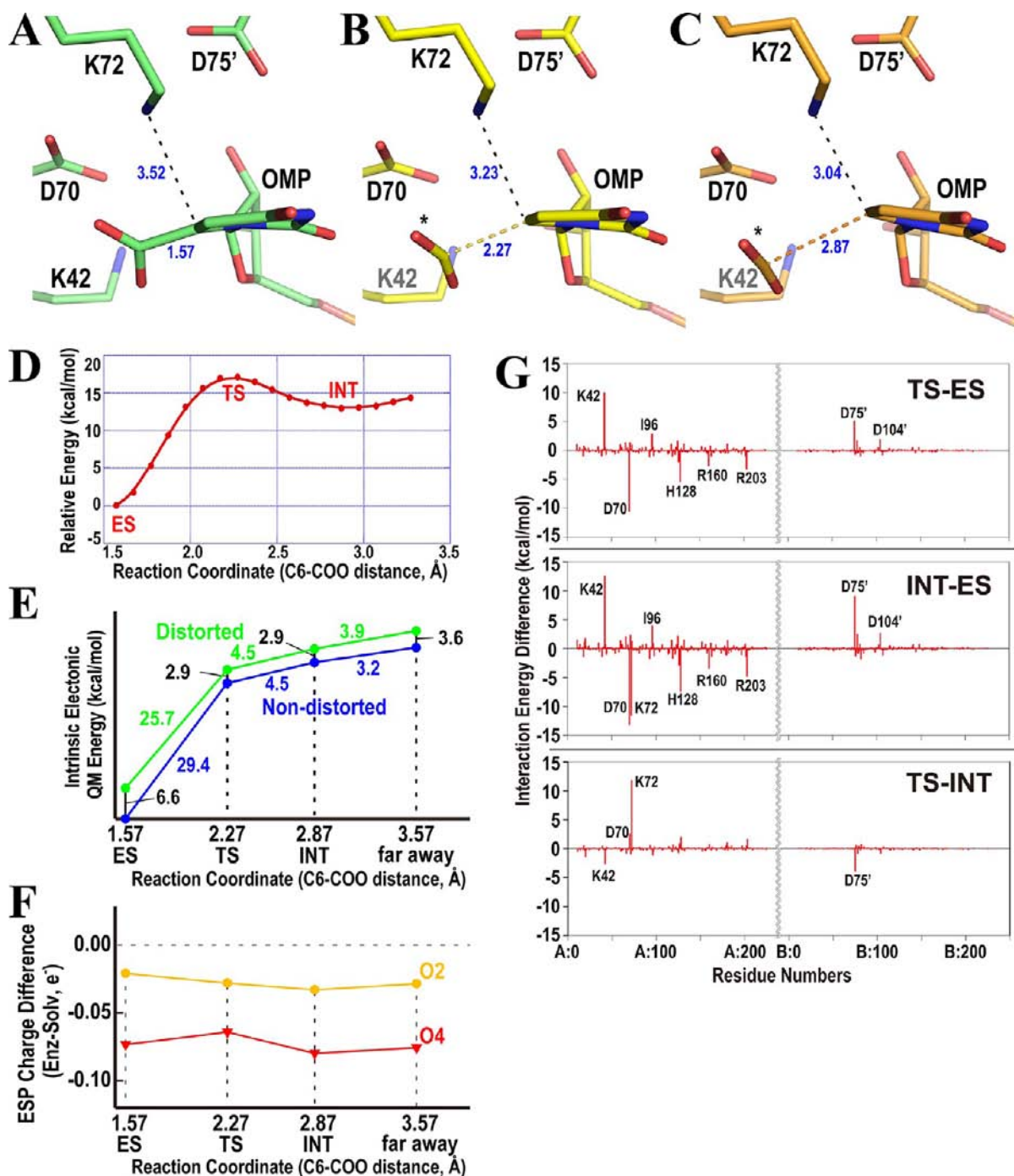
Figure 6. Simulations of the ODCase reaction. Representative structures of (A) enzyme–substrate complex (ES), (B) transition state (TS), and (C) intermediate state (INT) are drawn. The three states are defined in panel D. The asterisks represent the released carboxylate. (D) Direct decarboxylation profile forming vinyl anion intermediate along the reaction coordinate determined by ab initio QM/MM calculations (QM/MM MP2/6-31(+) G **//RHF/6-31(+) G **//AMBER (parm.96)). The x - and y -axes indicate the C6–COO bond distance (Å) and the relative energy of the reaction (kcal/mol), respectively. TS and INT are defined in the peak and the metastable part along the decarboxylation path, respectively. (E) Potential energy profiles of the electronic energy (QM energy) of the distorted (green, inside enzyme) and nondistorted (blue, in aqueous solution) orotate portion of the OMP substrate. The distorted energy penalty is implicitly incorporated into the potential energy curves, and these intrinsic energy profiles are mapped onto the reduced one-dimensional reaction coordinate as shown in panel D. The x - and y -axes indicate the reaction coordinate of the C6–COO distance and the relative energy of the decarboxylation reaction, respectively. Energy differences between the two profiles (numbered in black) represent the additional energy cost to deform the ligand structure relative to the reference, which is the relaxed structure in the aqueous solution. (F) Electrostatic potential (ESP) charge difference between enzyme-bound ligand and the ligand in solution. The x -axis indicates the reaction coordinate of the C6–COO distance. The y -axis indicates the ESP charges in enzyme subtracted by those in solution. The charges of all atoms in the pyrimidine ring are represented in Figure S3. (G) Interaction energy differences between two selected states along the decarboxylation coordinate determined by FMO2-RHF/6-31 G * calculations. Upper, middle, and lower panels indicate energy difference between TS and ES, between INT and ES, and between TS and INT, respectively. The x -axis corresponds to the amino acid residue serial number, and the y -axis designates the interaction energy differences between the two selected states.
