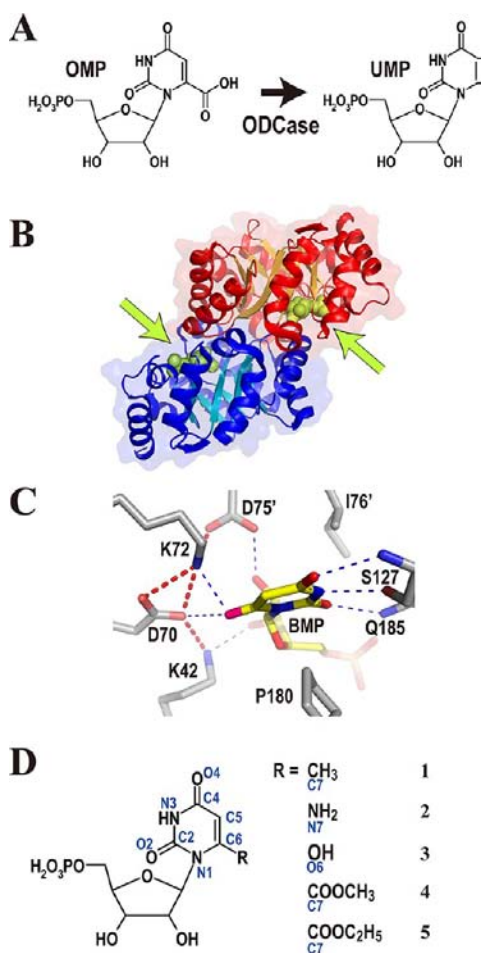
Figure 1. (A) Reaction catalyzed by ODCase. (B) Physiological dimer of MtODCase . The green arrows indicate the binding positions of the ligands, which are drawn as green spheres. (C) Electrostatic and hydrogen bond network in the active site of ODCase. WT- MtODCase complexed with BMP (PDB 1X1Z) is presented as an example. (D) Substrate analogues described in this paper. Atom numbering is shown in blue. 1, 6-methyl-UMP; 2, 6-amino-UMP; 3, BMP; 4, OMP-methyl-ester; 5, OMP-ethyl-ester.
